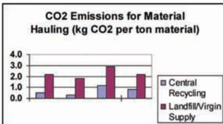
Figure 1: Comparison of CO 2 emissions in kg CO 2 per ton of material processed using central depot recycling compared to landfilling waste material and virgin aggregate supply for base stabilization.
