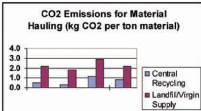
Figure 2: Comparison of CO2 emissions in kg CO2 per ton of material processed using on-site material recycling compared to landfilling waste material and virgin aggregate supply for base stabilization.
